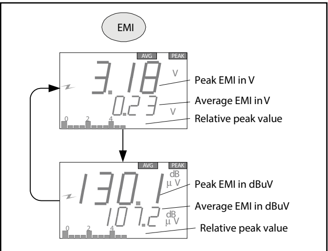
Figure 12. EMI Measurement screen
