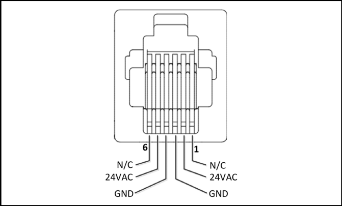
Figure 8. Pin-out of the console's power socket
